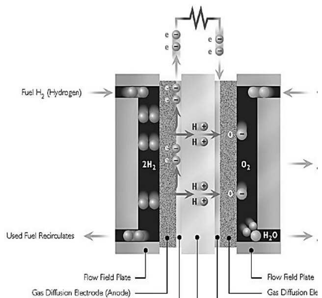
Figure 1 – The fuel element
