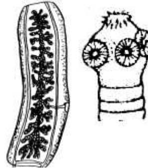
Mature proglottid and scolex Taenia multiceps
