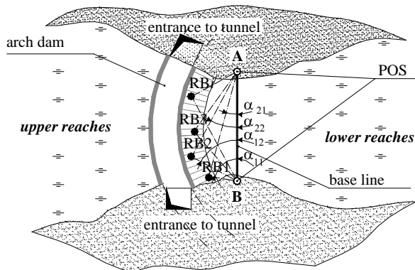
Fig.3. Placement of two vertical POSs for arch dam monitoring.
