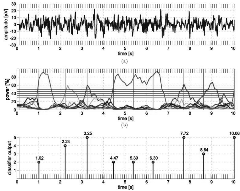
Figure 3 - Spelling with Bremen BCI in the example of subject 7 and the copy spelling word "BCI". The classifications were performed every 13 samples; these moments are marked with stroke lines on the x axes in the diagrams. (a) Example of the EEG signal acquired from site Oz (one of the eight electrodes used in this study). (b) Signal classification on the basis of different thresholds \beta_i , ranged from 30 to 50%. Each colour corresponds to the individual stimulating frequency and the related threshold \beta_i . (c) Classifier output.
