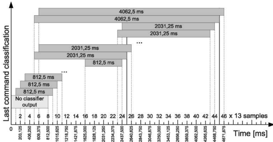
Figure 2 - Changes in the time segment length ( T_{Sn} ) after each performed classification in case no classification can be made at the moment and the actual time t allows the extension of the T_s to the next pre-defined value. The horizontal bars represent the EEG data currently used for classification.
