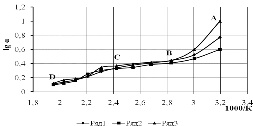
Figure 3.9 - Dependence of the logarithm of the degree of mass change on the biscuit semi-finished product temperature:
