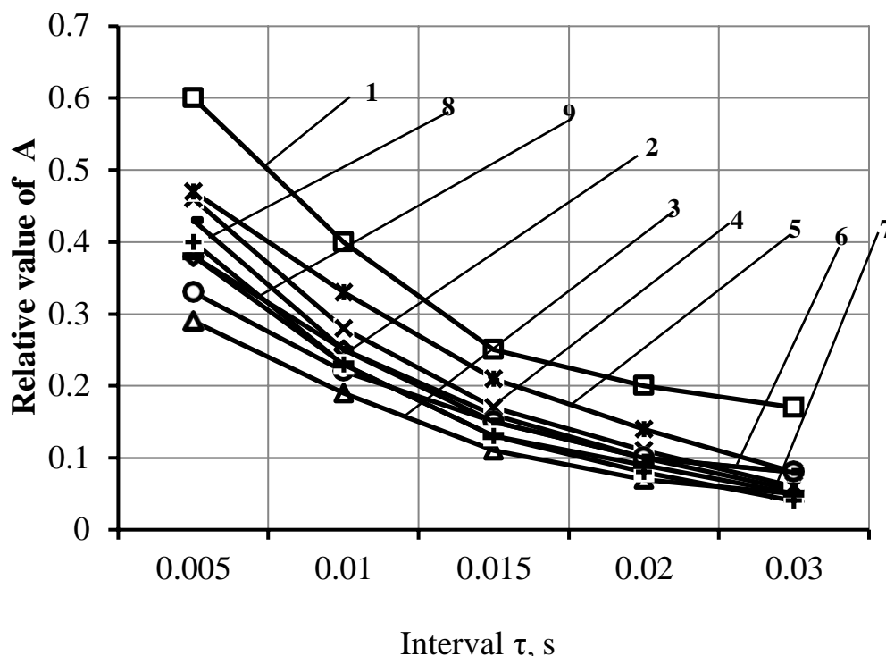
Figure 2.1 - Dependence of the amplitude of the spin echo signal from the interval \tau between pulses for biscuit dough samples using ECF:
