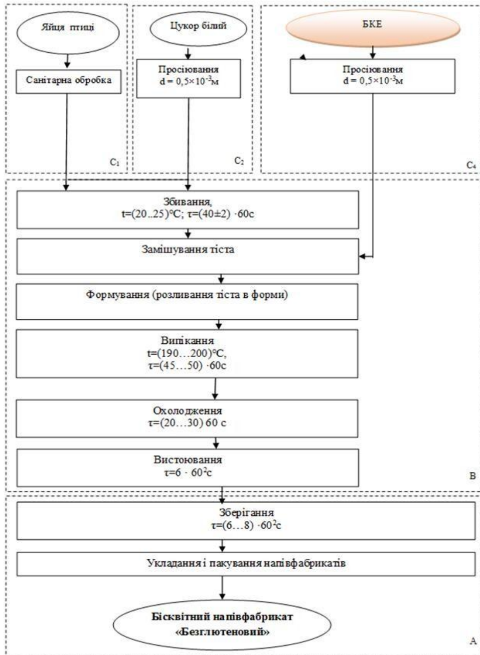
Figure 3.11 - Technological scheme of production of biscuit semi-finished product "Gluten-free" based on ECF
