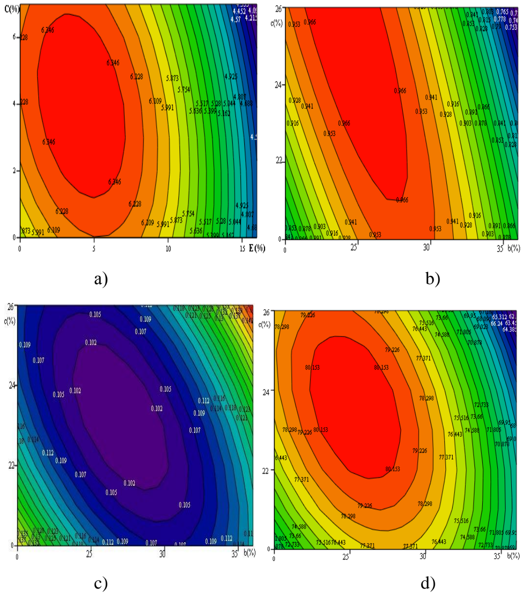
Figure 3.7 - Lines of density level (a), moisture content (b), baking (c) and porosity (d) of biscuit dough in relation to the parameters of eggs and sugar content
