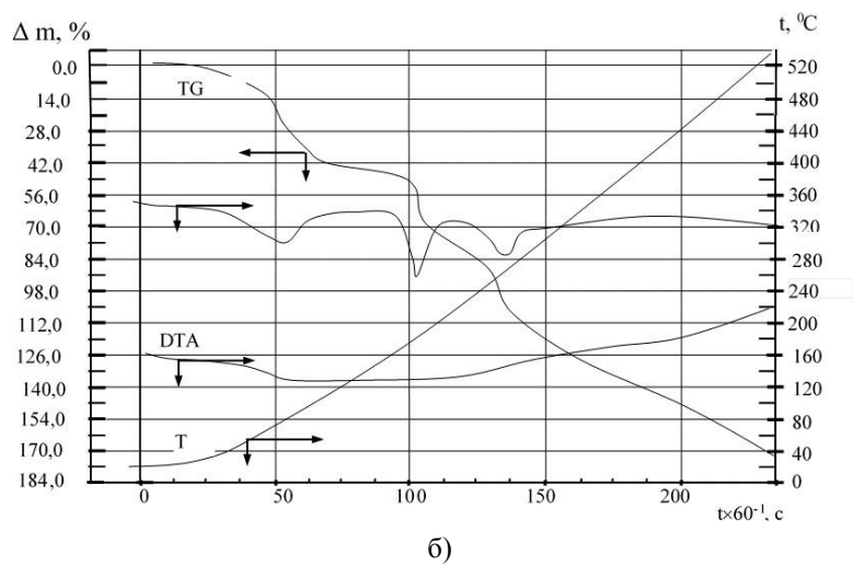
6) Figure A.3 - Derivatograms of biscuit semi-finished products after 72 \cdot 60 2s of storage: a) control; b) "Sun"
