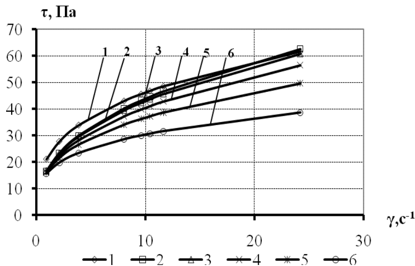
Figure 3.1 - Dependence of bias voltage, ( \tau , PA) on speed of shear, ( \gamma , s-1) for biscuit dough samples:
