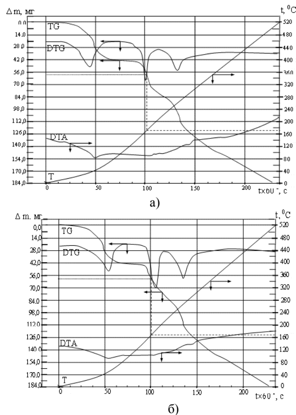
Figure A.1 - Derivatograms of biscuit semi-finished products after 24 · 60 2s of storage: a) control; b) "Sun"
