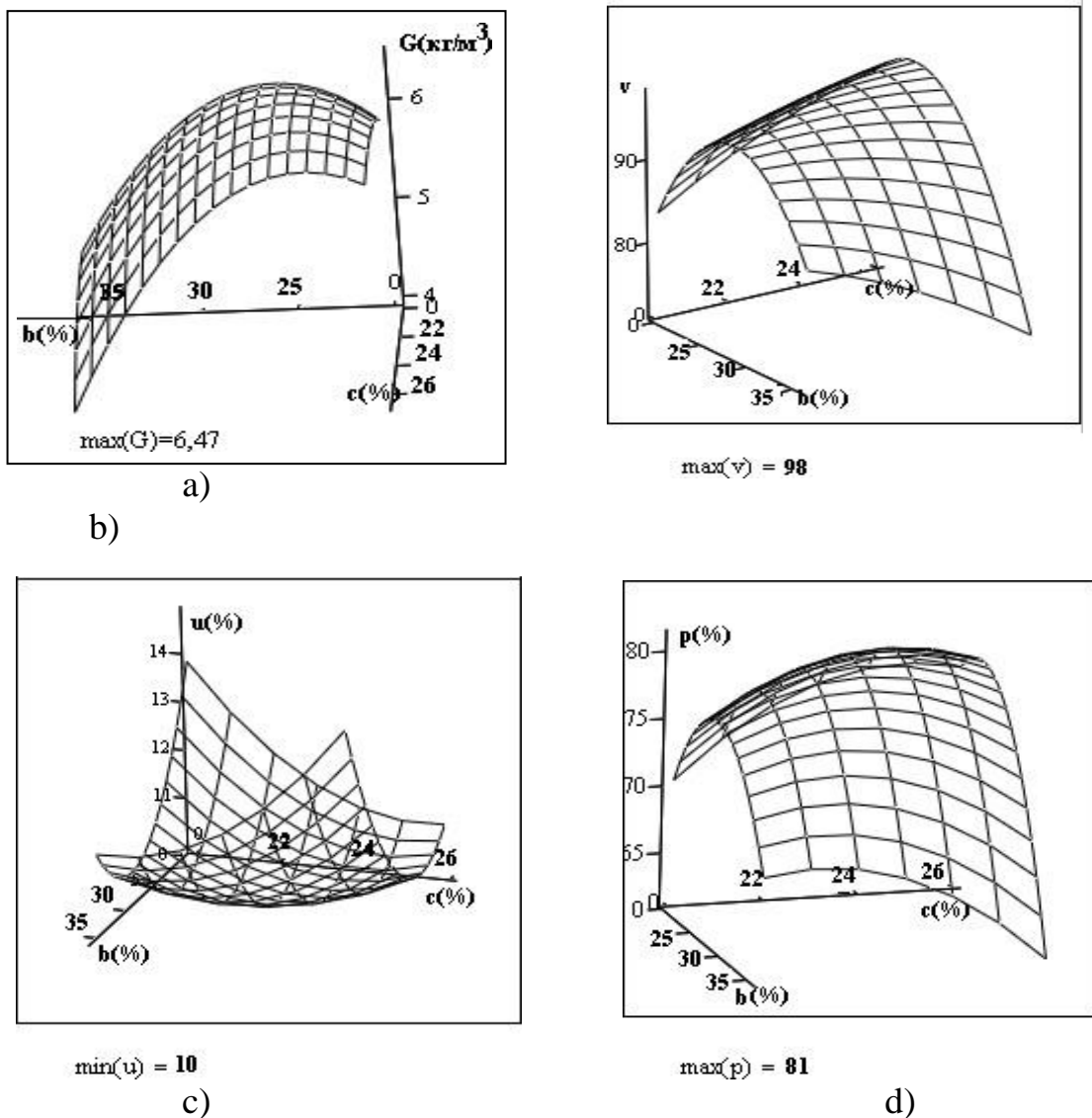
Figure 3.6 - Surfaces of the dependence of density (a), moisture content (b), baking (c) and porosity (d) on the content of eggs products and sugar biscuit dough
