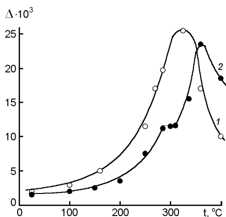
Fig. 1. Temperature dependences of IF for quenched 60C2A steel at heating in the range of 0 to 400°C. The initial state: non-deformed specimen (1), deformed at \varepsilon = 30\% , deformational aging at 350°C (2).
